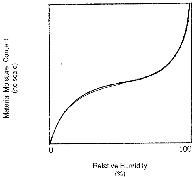
Figure 2 — Relationship of Material Moisture Content to Relative Humidity of Surrounding Air
