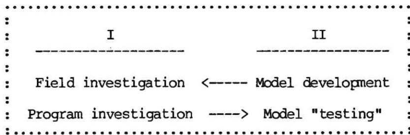
Figure 1. Project Process.
